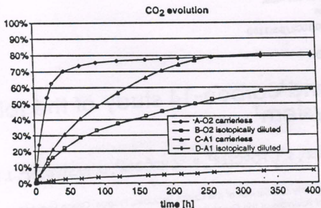
Figure 1 Microbial degradation of [1,2- ^{14}\text{C} ]TCA in spruce-forest soil (horizon A and O2) amended with 396 kBq of [1,2- ^{14}\text{C} ]TCA, i.e. with 17.5 (carrier-free) and 192 \mu\text{g} (11 times isotopically diluted) TCA, in 50 g soil at the beginning; the curves show influence of soil character on the released ^{14}\text{CO}_2 in the course of degradation at room temperature and 30% soil moisture; residual soil radioactivity corresponds mostly to microorganisms biomass. At the end (after 17 days) the soil contained only 0.7 kBq [1,2- ^{14}\text{C} ]TCA from 76.4 kBq residual ^{14}\text{C} -activity determined by combustion method (or 81.2 kBq estimated by subtraction of the released ^{14}\text{CO}_2 from the sample). The major part of the residual ^{14}\text{C} -activity of experiments A and C belongs to radioactive microbial biomass, less than 0.5% radioactivity (about 220 Bq) was found as oxalic acid. The degradation rate is substantially influenced by TCA level and soil character.
